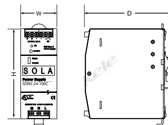
SDN-C Series Dimensions
